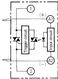
Terminal Arrangement/ Internal Connections
