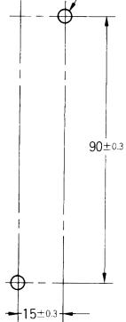
Mounting Holes
