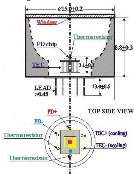
Package TO-5 with Parabolic Reflector
