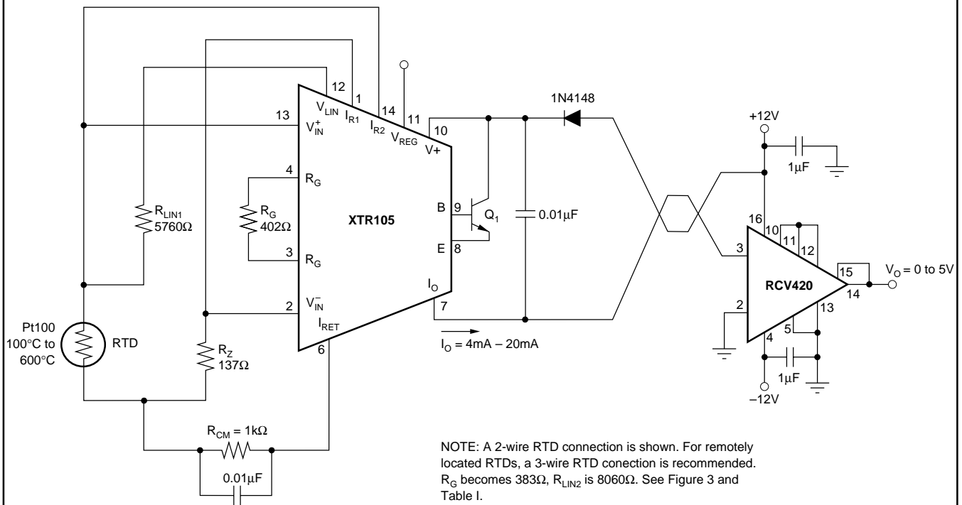
FIGURE 7. ±12V Powered Transmitter/Receiver Loop.
