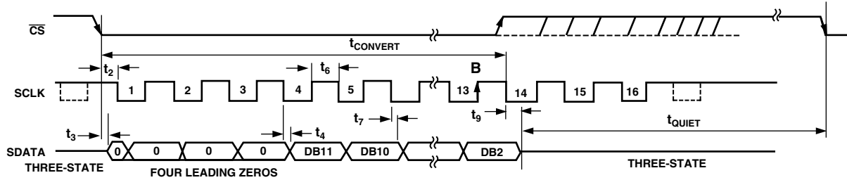
Figure 21. Serial Interface Timing Diagram—Conversion Termination
