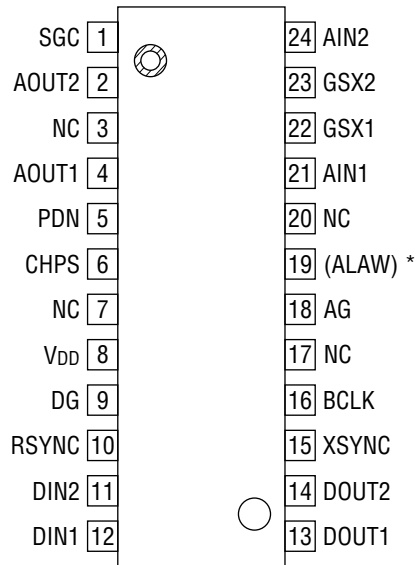
24-Pin Plastic SOP
