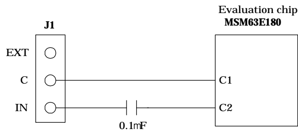
Figure 2-20 Jumper 1 Circuit
