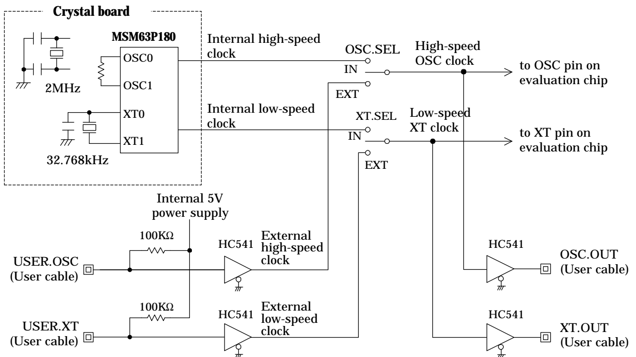
Figure 2-17 Clock Circuits
