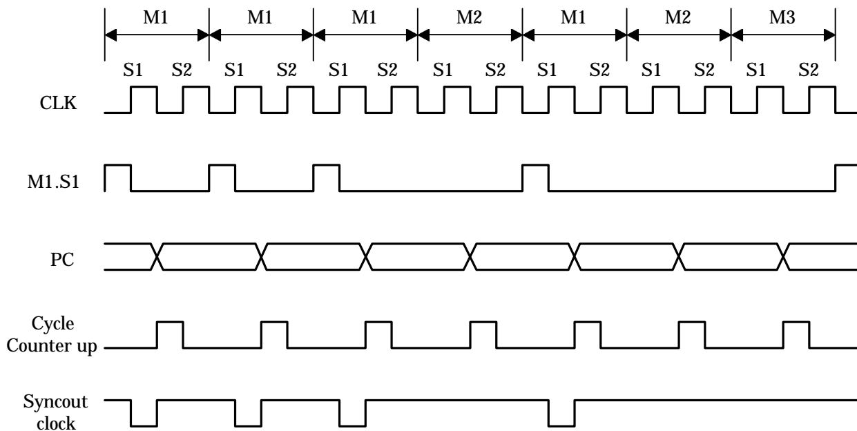
Figure 4-2 Cycle Counter/Sync Out Timing Chart
