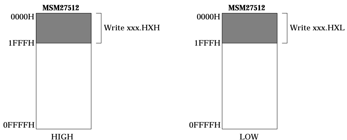
Figure 2-1 Address Ranges for MSM27512
