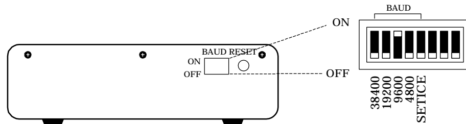
Figure 2-22 BAUD Switch
