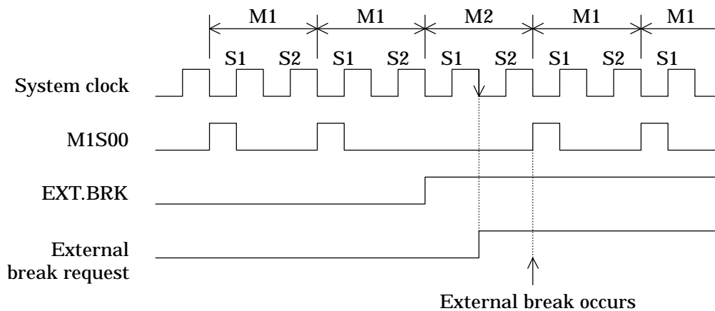
Figure 2-13 External Break Input Timing
