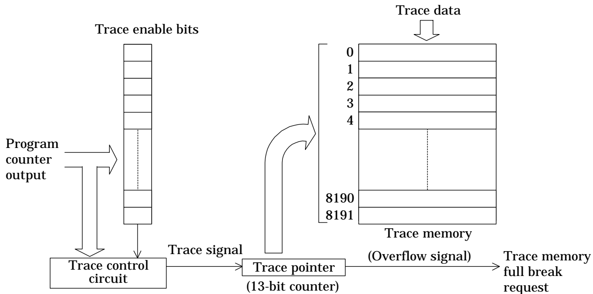
Figure 2-8 Real-Time Tracing
