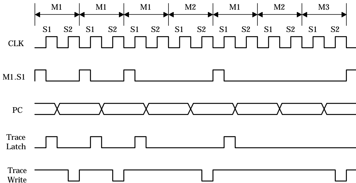
Figure 4-1 Trace Timing Chart
