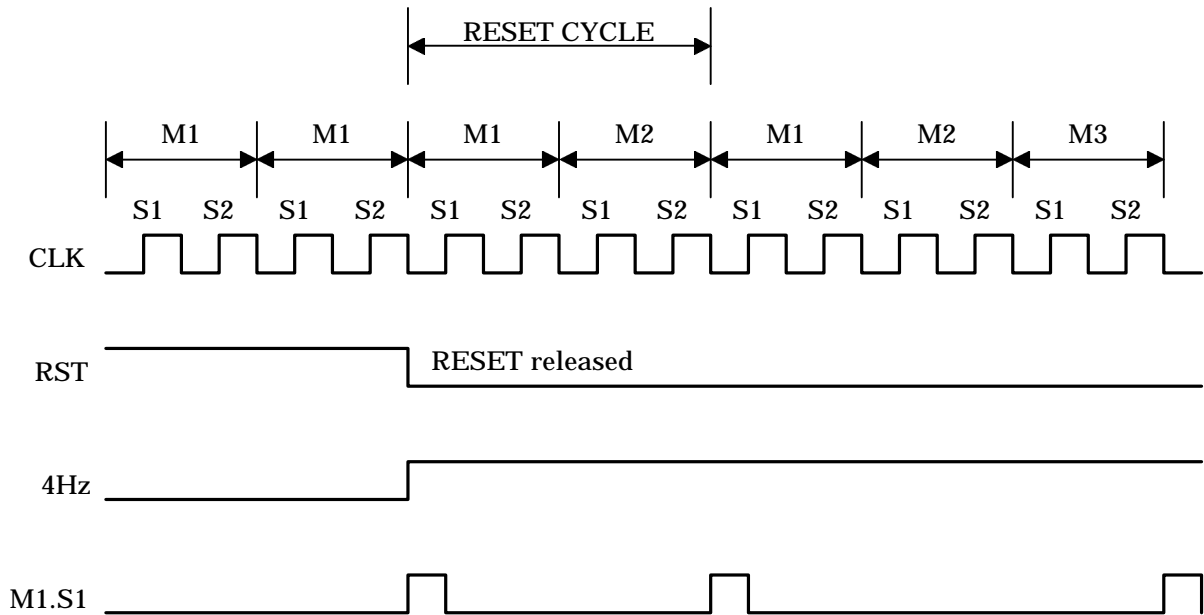
Figure 4-3 Reset Timing Chart
