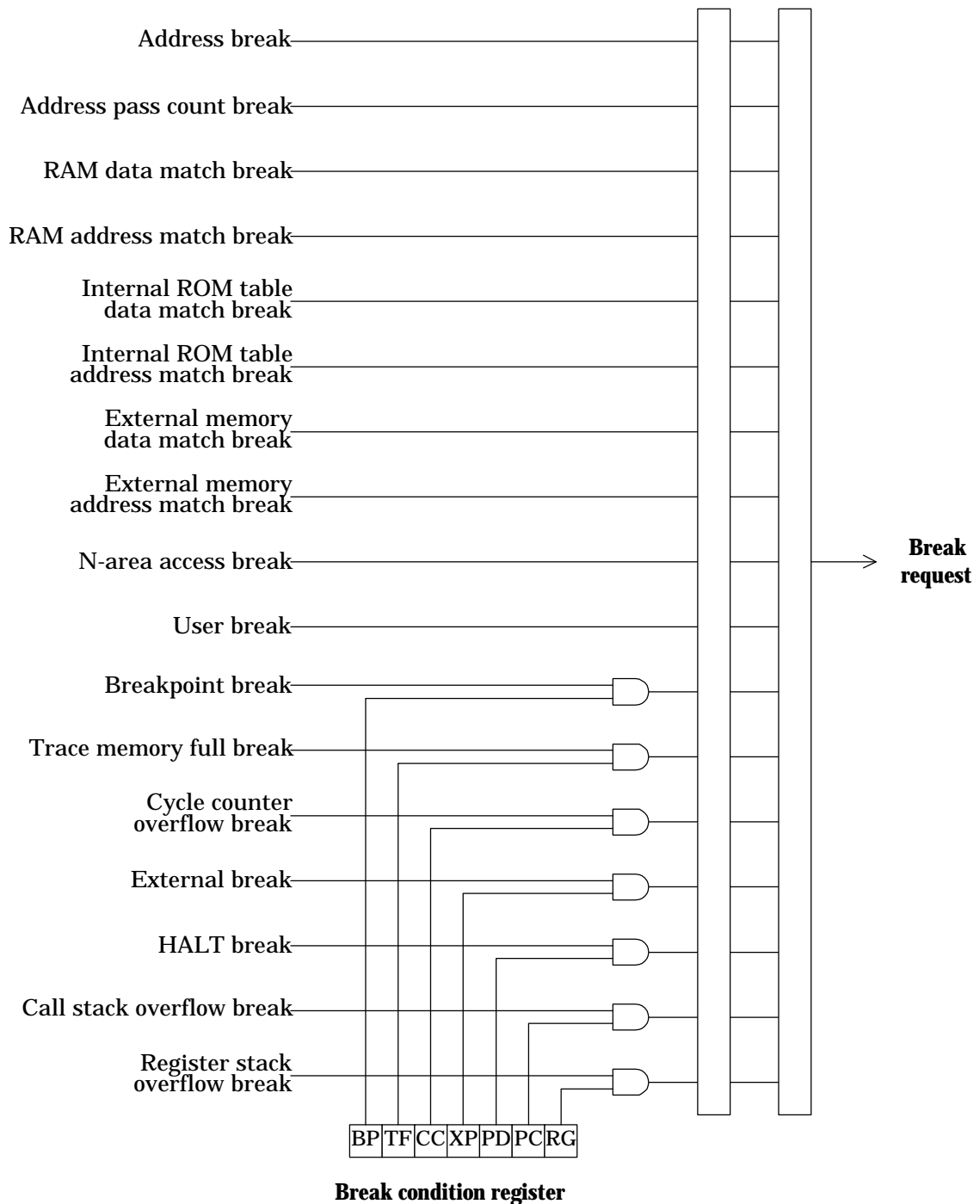
Figure 2-3 From Break Condition to Break Request
