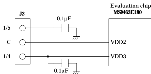
Figure 2-21 Jumper 2 Circuit
