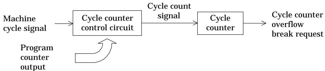
Figure 2-11 Cycle Counter
