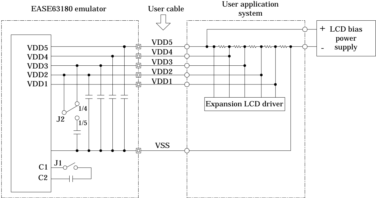
Figure 3-3 Interface Example for Expansion LCD Driver with External Bias Power Supply
