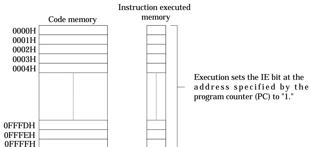
Figure 2-10 IE Bits
