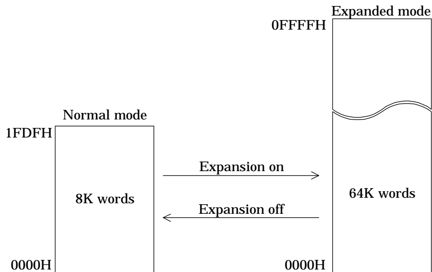
Figure 2-6 Code Memory Expansion
