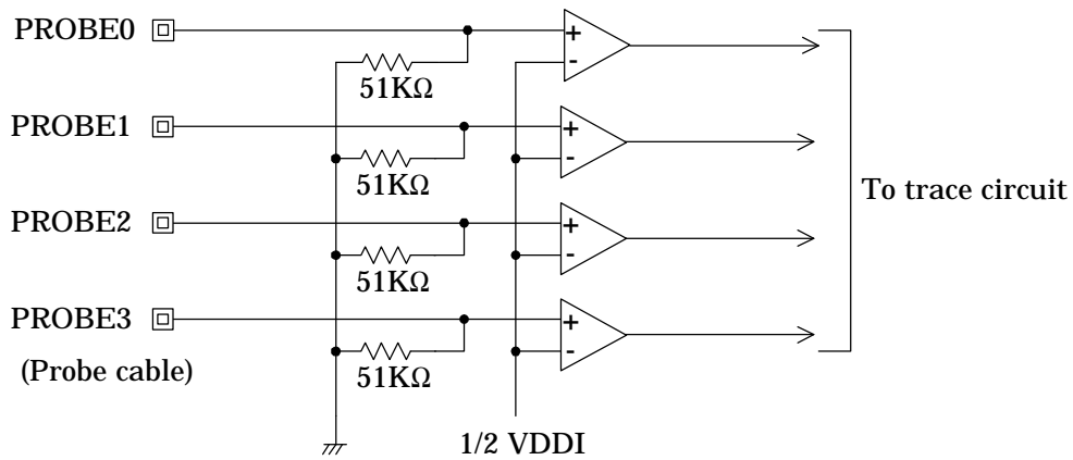
Figure 2-15 Trace Inputs
