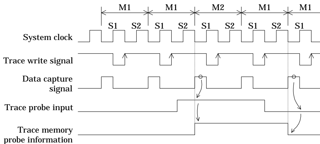
Figure 2-16 Trace Input Timing
