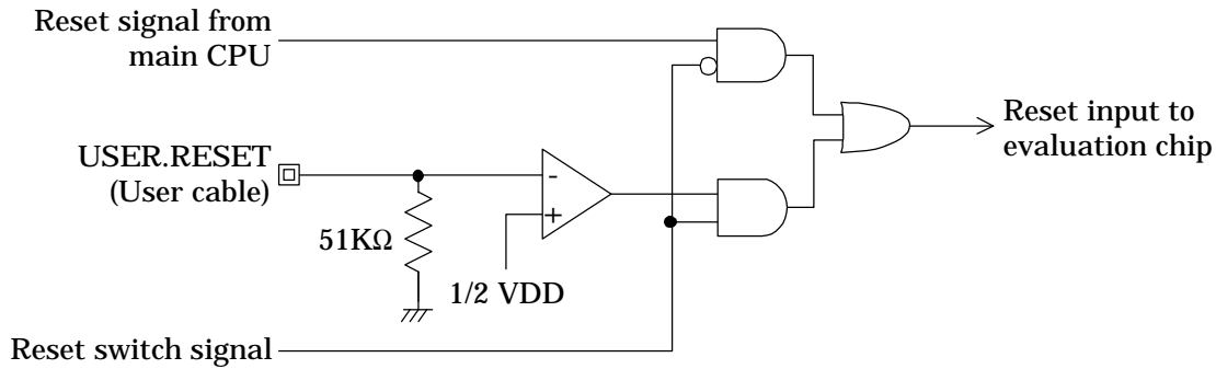
Figure 2-19 Reset Input
