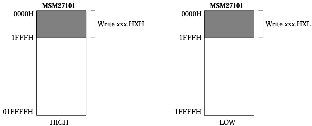
Figure 2-2 Address Ranges for MSM27101
