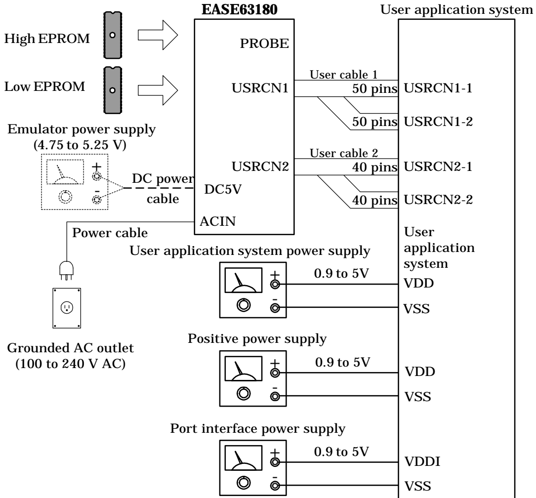
Figure 3-4 Connections for Emulation
