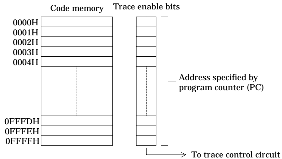
Figure 2-9 Trace Enable Bits
