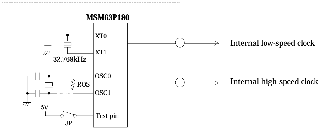
Figure 2-18 Crystal Board Circuits
