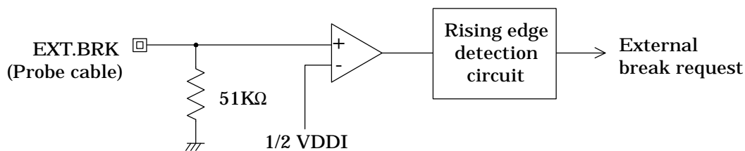
Figure 2-12 Break Signal Input
