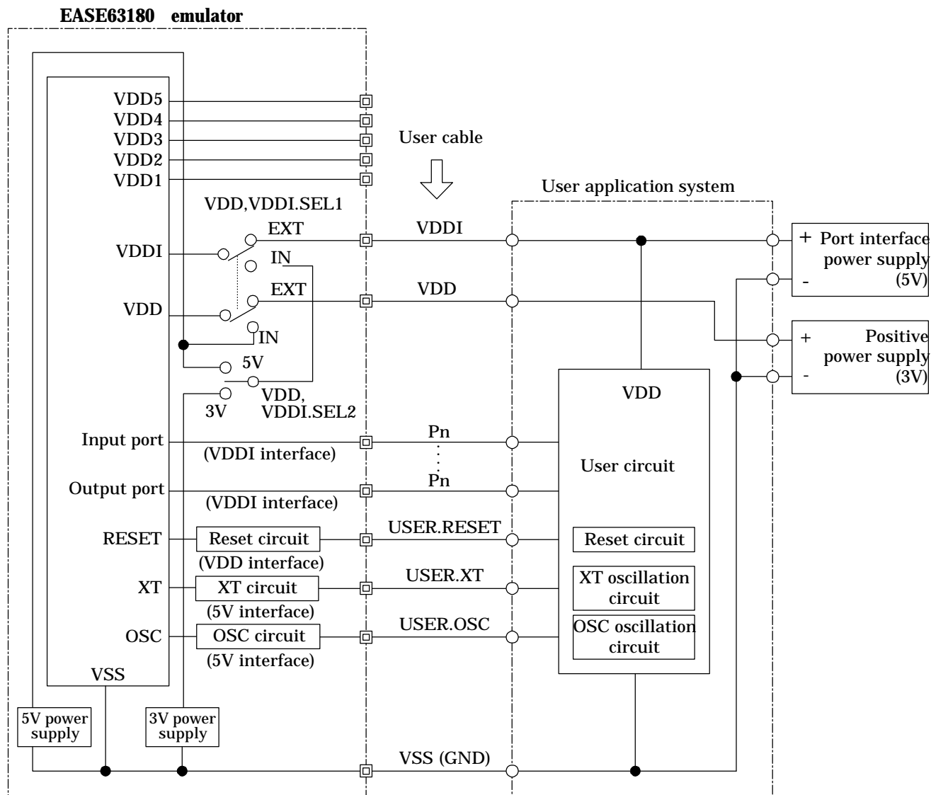
Figure 3-2 Power Supply Interface Example
