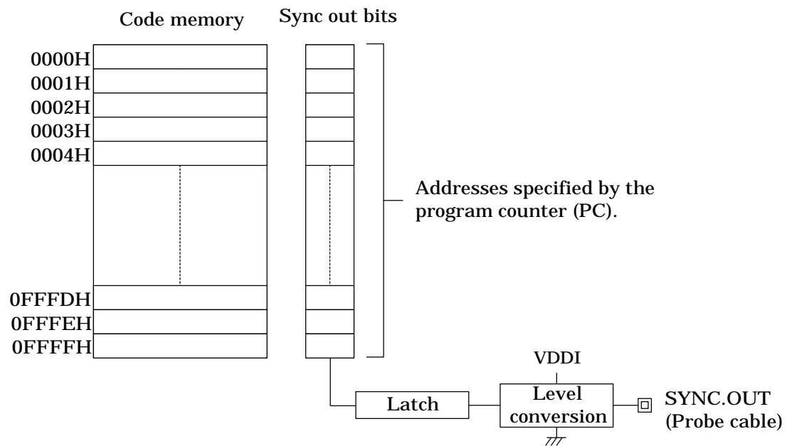
Figure 2-14 Sync Out Bits
