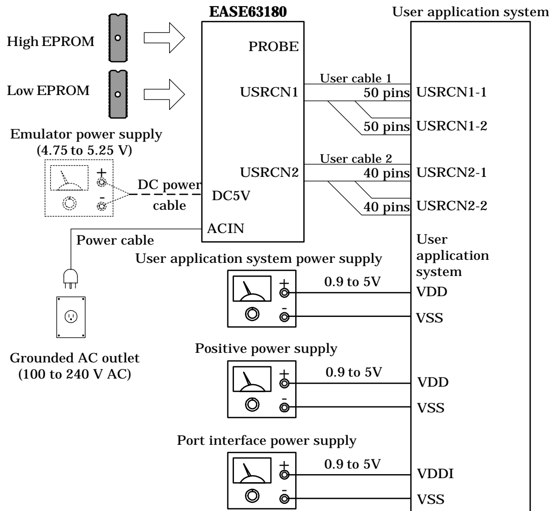
Figure 3-1 Connections for Evaluation
